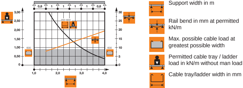
Load diagram, LG 60 NS
