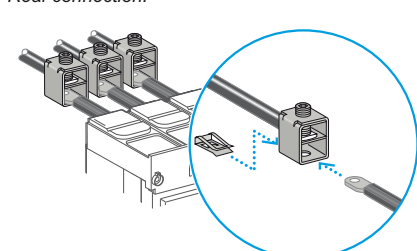
Connection of bare cables to NSX100 to 250.
