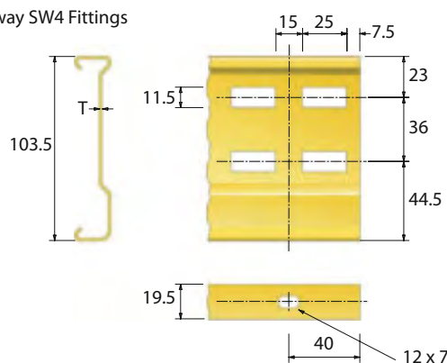
Speedway SW4 Fittings
