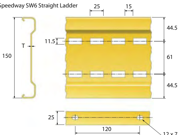
Speedway SW6 Straight Ladder
