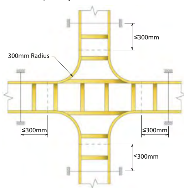
Speedway Crosses (300mm Radius)
