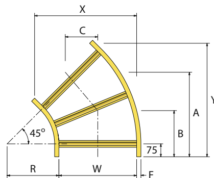
Speedway 45° Flat Elbows
