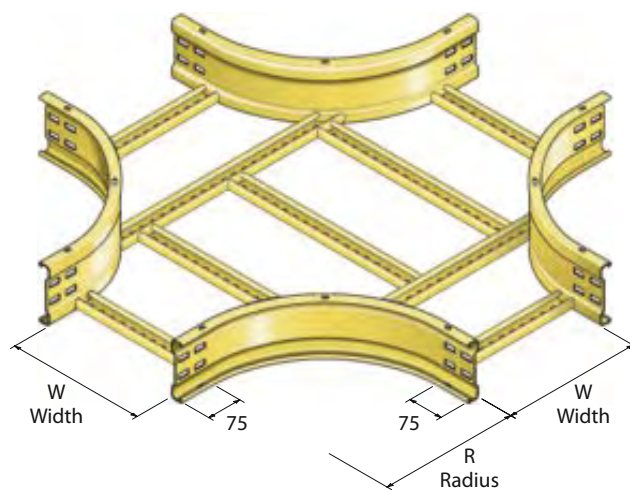
Speedway Cross All branches have identical widths
