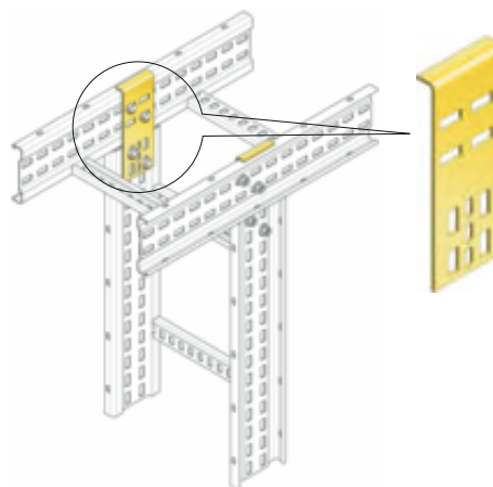
Speedway drop out bracket securing a vertical cable ladder to a horizontal cable run
