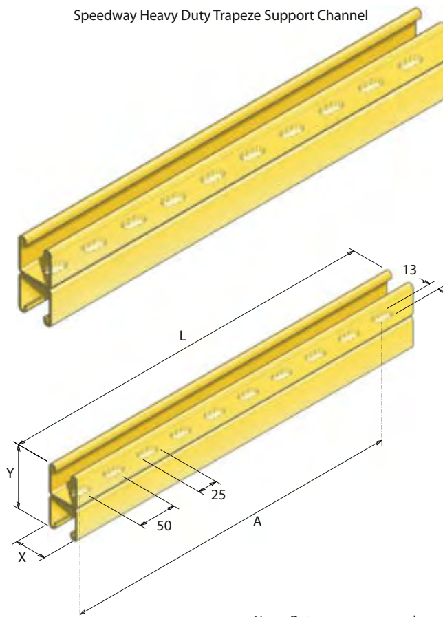
Heavy Duty trapeze support channel suspended on M10 threaded rod and supporting Speedway SW5 cable ladder
