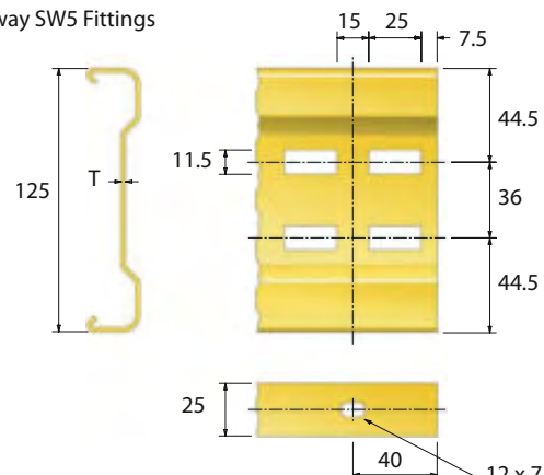
Speedway SW5 Fittings
