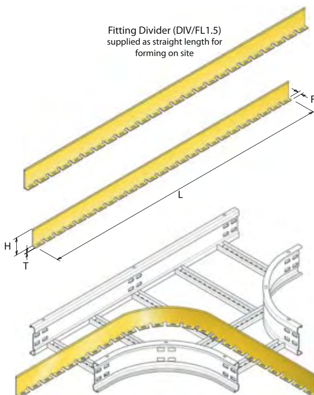
Fitting divider as installed on a Speedway tee fitting
