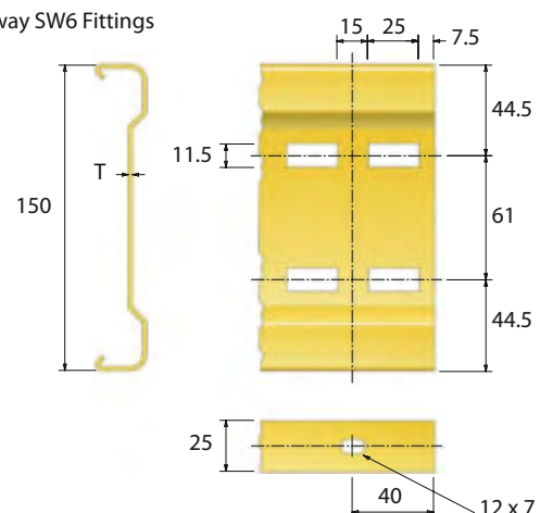
Speedway SW6 Fittings
