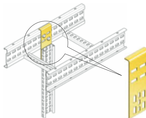
Speedway drop out bracket securing a vertical cable tray to a horizontal cable run
